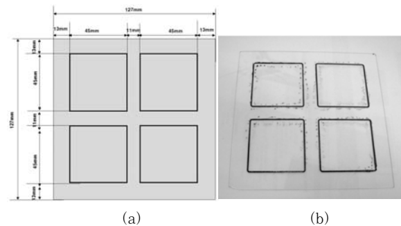
Fig. 2 Printed frit on the glass (a)pattern and (b)sample
