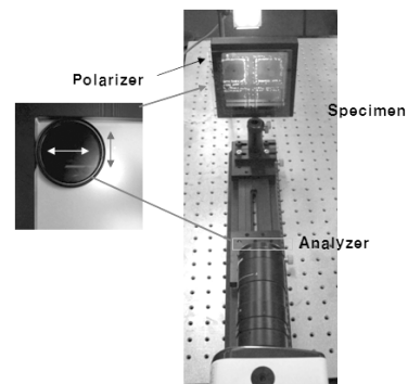
Fig. 6 photo-elasticity test device
