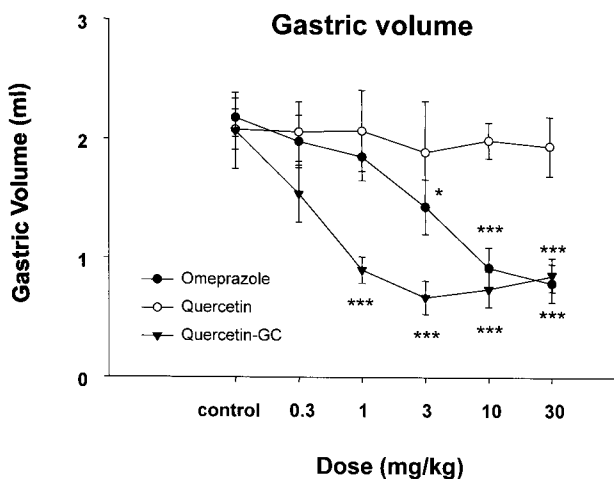
Fig. 2. The effect of QGC on gastric volume. QGC significantly and dose-dependently decreased gastric volume. Data are means±SEM. *p<0.05, **p<0.01, and ***p<0.001 vs. the control (n=6~8).
