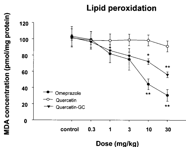
Fig. 5. The inhibitory effects of QGC on lipid peroxidation. In the gastritis control group levels of lipid peroxidation were elevated as compared with the normal group. QGC administration significantly decreased the amount of MDA formation, suggesting that it inhibited gastritis induced lipid peroxidation. Column represent means \pm SEMs of 6~8 animals. * p <0.05 and ** p <0.01 vs. control.
