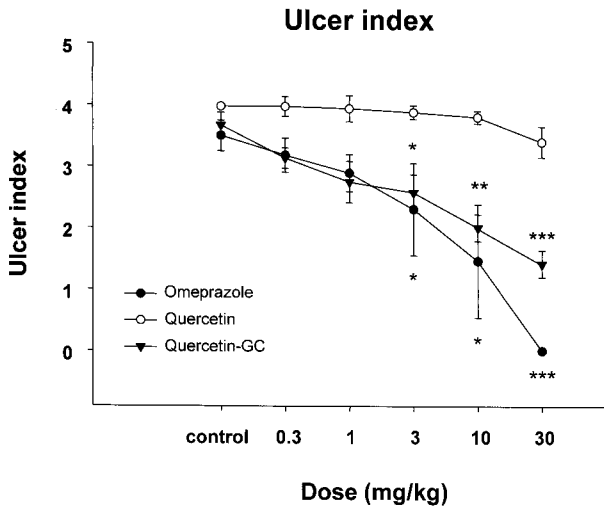
Fig. 1. The effect of QGC on reflux esophagitis induced surgically in rats. Mean lesion area in the control group was 4 (0, no lesion; 1, ulcer area; 2, ulcer area < 30 mm 2 ; 3, ulcer area > 30 mm 2 ; 4, complete lesion (perforation of the esophageal mucosa). QGC treated animals showed significantly inhibition on reflux esophagitis. Data are means±SEMs of 6~8 animals. *Significantly different from the corresponding controls. *p<0.05, **p<0.01, and ***p<0.001 vs. the control.
