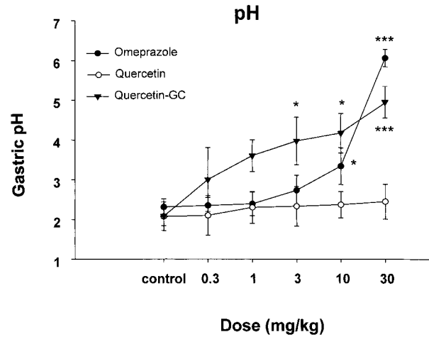
Fig. 3. The effects of QGC on gastric pH. QGC administration changed the pH of reflux esophagitis in rats. QGC significantly increased when compared with the pH of quercetin. Data are means±SEM. *p<0.05, ***p<0.001 vs. the control (n=6~8).
