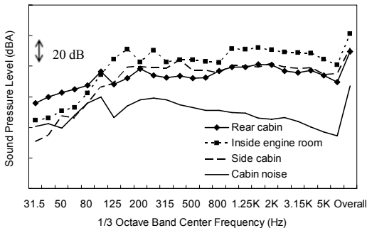
Fig. 10 Excavator's noise source levels
