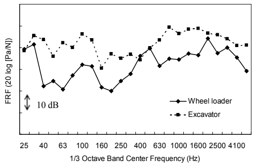
Fig. 8 FRF of structureborne noise transmission
