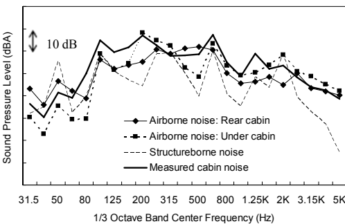
Fig. 12 Noise transmission paths in wheel loader's cabin
