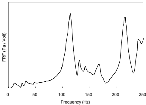
Fig. 15 Acoustic excitation test results of wheel loader
