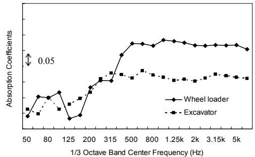
Fig. 2 Absorption coefficients of cabins
