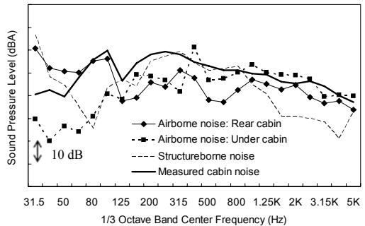
Fig. 13 Noise transmission paths in excavator's cabin
