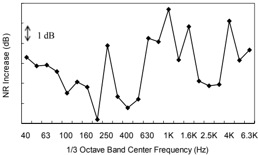
Fig. 14 NR increase by removing flanking noise
