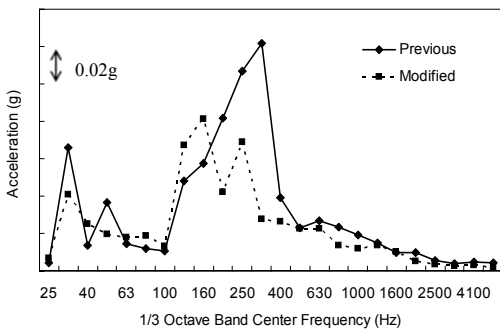
Fig. 16 Comparison of vibration levels at cabin mounts
