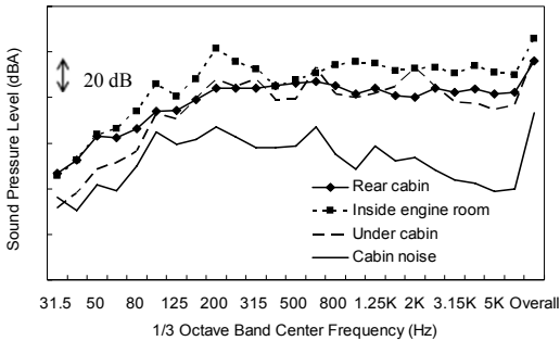
Fig. 9 Wheel loader's noise source levels
