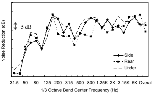
Fig. 6 NR of excavator's cabin
