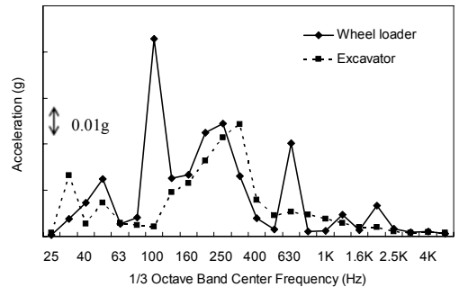
Fig. 11 Vibration levels measured at cabin mounts
