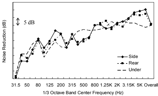
Fig. 5 NR of wheel loader's cabin
