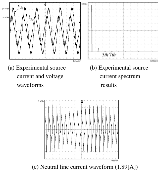
Fig. 6. Waveforms for the harmonic current source when compensated with the parallel passive filter.
