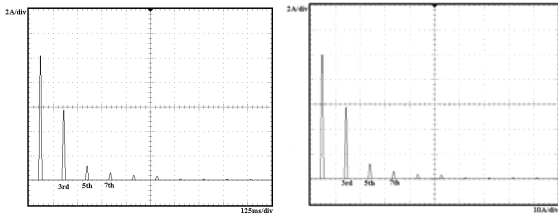
(c) Experimental source current spectrum result under balanced load condition (THD : 57.6%) (d) Experimental source current spectrum result under un-balanced load condition (THD : 59.2%)
