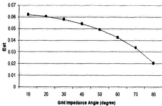
Fig. 7. Variation of short term voltage flicker severity E_{st} with grid impedance angle \psi_k . ( SCR = 20, v = 9 m/s)
