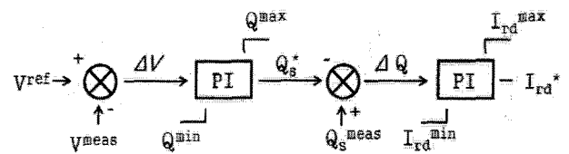
Fig. 14. Block diagram for voltage control through RSC.
