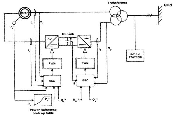
Fig. 11. Schematic diagram of the wind turbine system with STATCOM connected.
