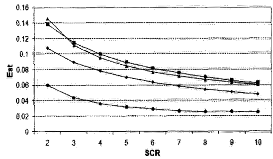
Fig. 8. Variation of short term voltage flicker severity E_{st} with SCR, reactive power set to: zero (square), 0.1 p.u. (diamond), 0.3 p.u. (circle), 0.5 p.u. (triangle). ( \psi_k=60^\circ, v = 9 m/s)
