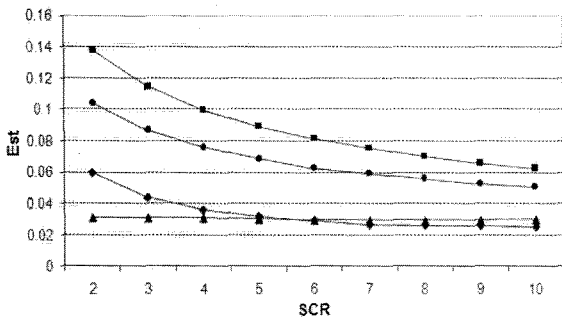
Fig. 17. Variation of short term voltage flicker severity E_{st} with SCR, reactive power set to zero (square), 0.3 p.u.(diamond), STATCOM ON (circle), voltage control mode (triangle). ( \psi_k = 60^\circ , v = 9 m/s)
