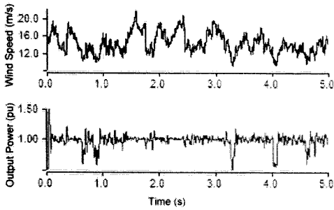
Fig. 5. Wind profile and corresponding output power of the wind turbine in the base case, but mean wind speed changed to 15 m/s.
