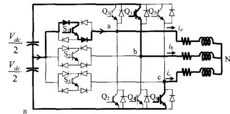
Mode viii; v_{an}=\frac{V_{dc}}{2}; v_{bn}=V_{dc}, v_{cn}=0
