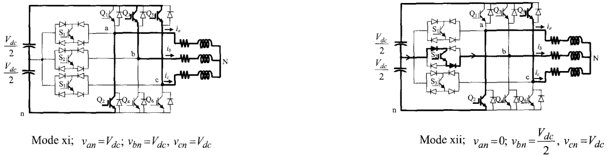
Fig. 4. Operational states of switches according to the switches on-off conditions.
