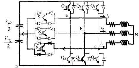
Mode iv; v_{an}=V_{dc}; v_{bn}=0, v_{cn}=\frac{V_{dc}}{2}
