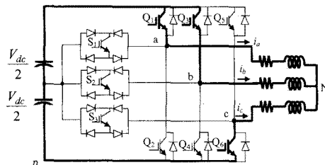
Mode vii; v_{an}=V_{dc}; v_{bn}=V_{dc}, v_{cn}=0
