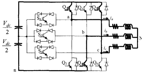
Mode iii; v_{an}=V_{dc}; v_{bn}=0, v_{cn}=V_{dc}
