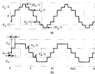
Fig. 6. MATLAB SIMULINK simulated waveforms of: (a) the load phase voltage waveform v_{an} and (b) the line-to-line voltage waveform v_{ab} .
