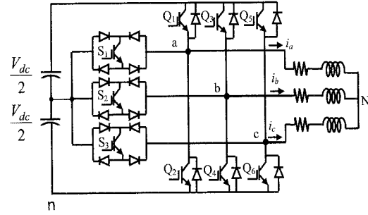
Fig. 2. The proposed nine switch three-level inverter.
