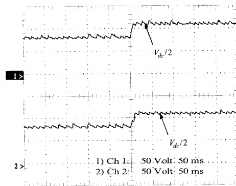
Fig. 10. The inverter dc bus voltages (50V/div, 50ms/div).
