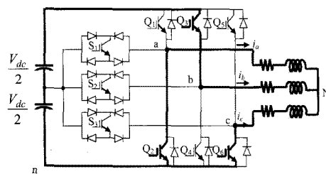
Mode ix; v_{an}=0; v_{bn}=V_{dc}, v_{cn}=0
