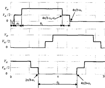
Fig. 5. MATLAB SIMULINK simulated waveforms of the load node voltages v_{an}, v_{bn} and v_{cn} .
