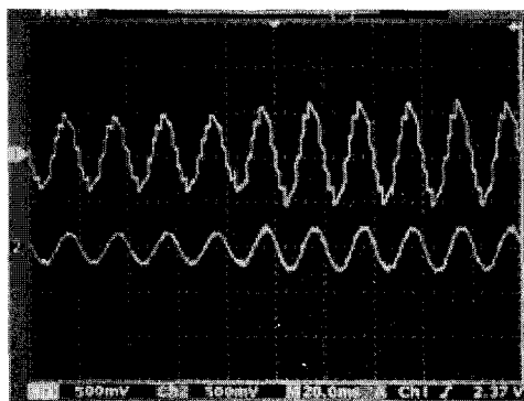
Fig.12. The load phase voltage v_{aN} and the line current i_a (150V/ div, 5Amp/ div, 20ms/ div).
