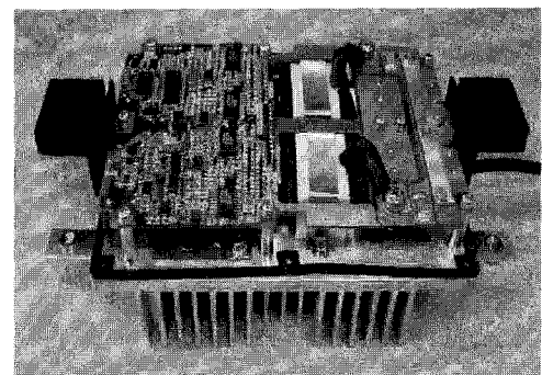
(a) 700W prototype with heat sink
