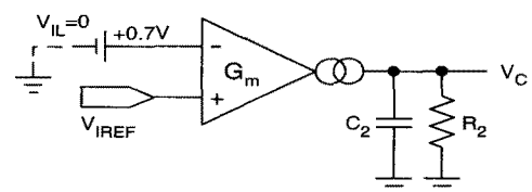
Fig. 8. Error Amp during gate block.
