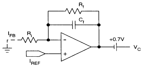
Fig. 10. Voltage mode error amplifier during blocking.
