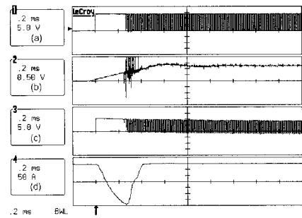
(a) Transient current without blocking time during startup
