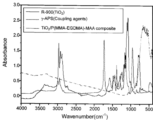
Figure 6. FT-IR spectra of \text{TiO}_2 and \text{TiO}_2/\text{P}(\text{MMA-EGDMA})-\text{MAA} .
