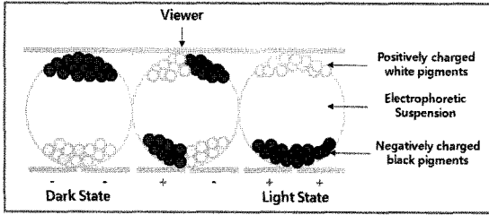
Figure 1. Scheme of microcapsule-type electrophoretic display.
