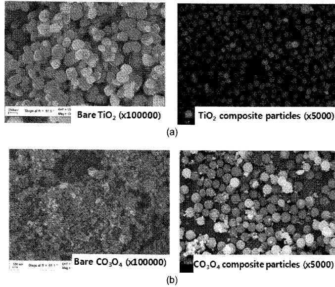
Figure 5. SEM photographs of white (a)/black (b) particles.
