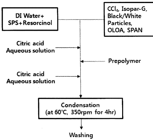
Figure 2. Procedure for prepolymer preparation and microencapsulation.
