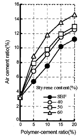
Figure 3. A/C of PMM.
