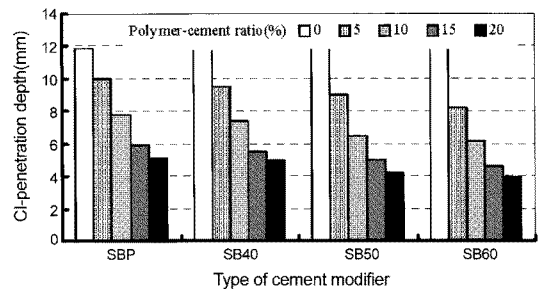
Figure 7. Chloride ion penetration of PMM.
