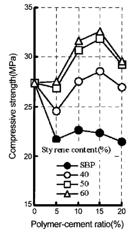
Figure 5. Compressive strength of PMM.
