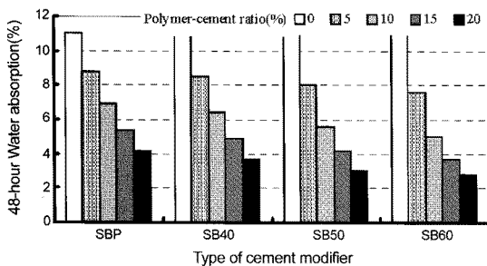
Figure 6. Water absorption of PMM.
