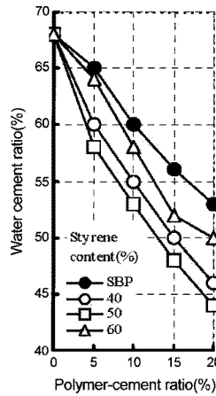
Figure 2. W/C of PMM.
