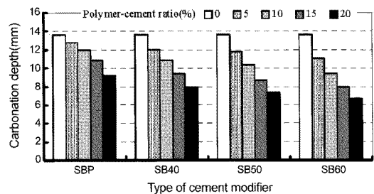
Figure 8. Carbonation depth of PMM.
