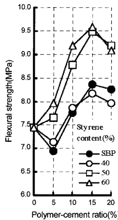
Figure 4. Flexural strength of PMM.
