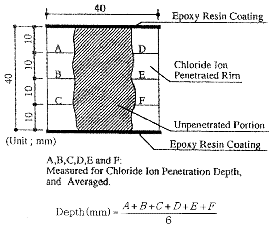
Figure 1. Cross section of specimen after chloride ion penetration test.
