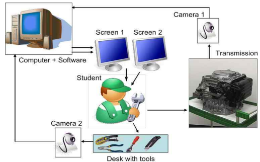
Fig. 4. Structure of developed training system
