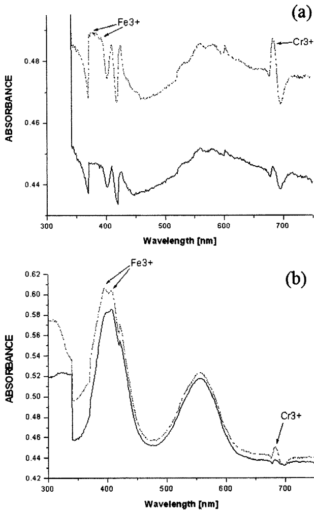
Fig. 4. The UV-VIS absorption spectrum of (a) SFNCS4, (b) SFPCS5.
