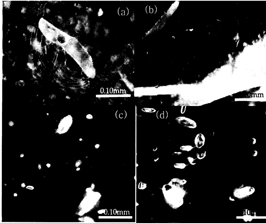
Fig. 5. (a) Stress fracture inclusion of flux sapphire (SFNCS 3), (b) Stress fracture inclusion of flux sapphire (SFNCS 4), (c) Stress fracture inclusion of natural sapphire (NNCS 2), (d) Stress fracture inclusion of natural sapphire (NPSC 2) ( \times 100 ).
