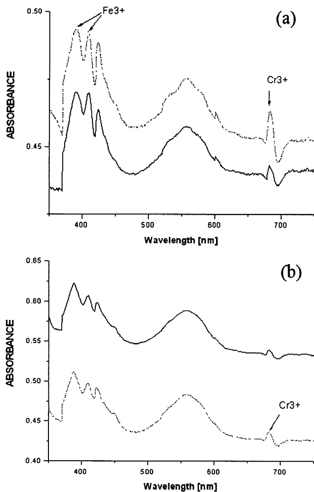
Fig. 2. The UV-VIS absorption spectrum of (a) NNCS3, (b) NPCS2.
