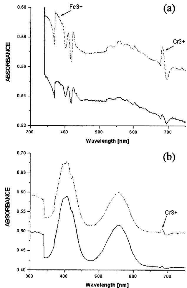
Fig. 3. The UV-VIS absorption spectrum of (a) SFNCS1, (b) SFPCS1.
