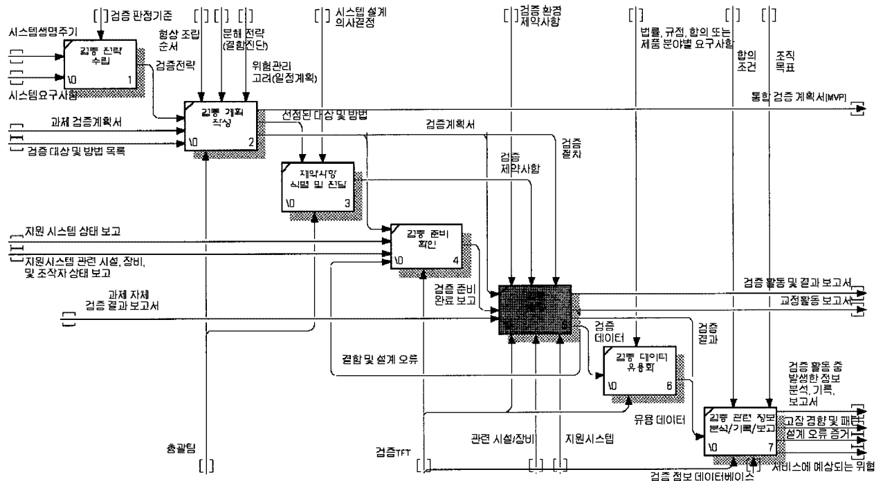
Fig. 5. Details of the Product Verification Process
