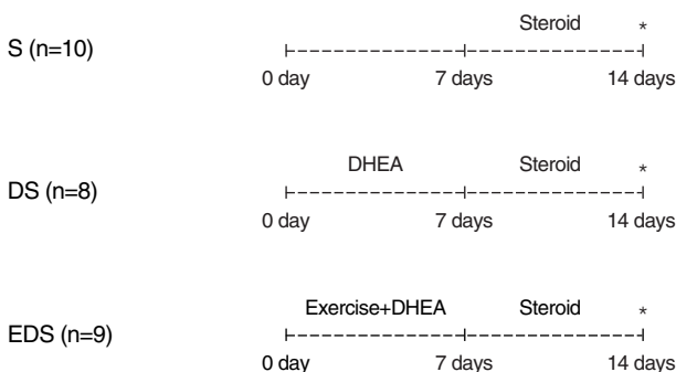
Figure 1. Experimental design.
