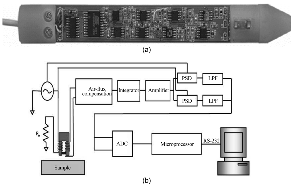
Fig. 2. (a) New eddy current test probe and (b) Block diagram of the measuring system.
