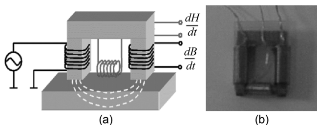
Fig. 1. (a) Structure of the sensor for magnetic phase detection, and (b) Photograph of the sensor.
