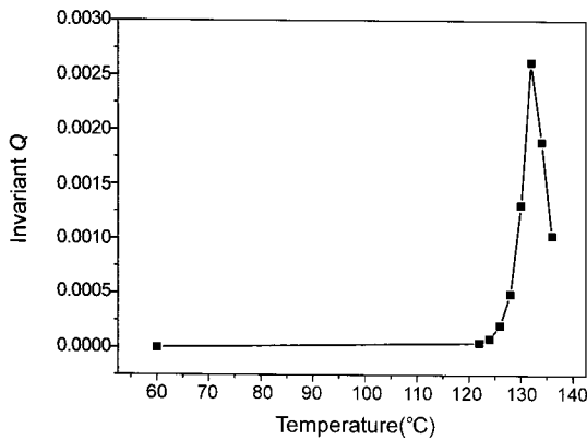
Figure 3. Invariant change of oriented HDPE.
