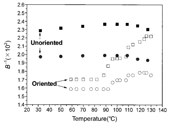
Figure 4. Change of peak width of HDPE samples. ■, □; (110) and ●, ○; (200).
