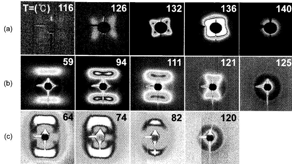
Figure 2. 2-D SAXS patterns of oriented (a) HDPE; (b) LLD-A; (c) LLD-B at corresponding temperatures.
