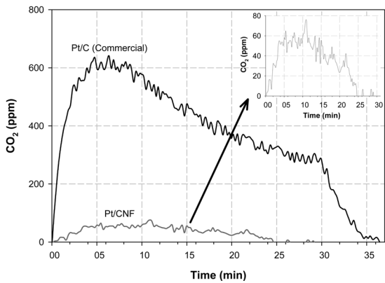
Fig. 3. Comparison of CO 2 mass-spectra profiles for MEAs with commercial Pt/C and Pt/CNF at 1.4 V for 30 min.
