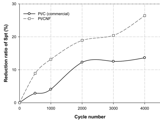
Fig. 7. Comparison of Pt active surface area loss for the commercial Pt/C and Pt/CNF at different cycle numbers during CV test.
