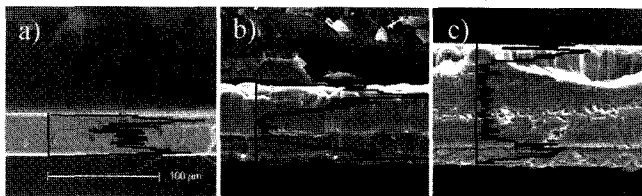
Figure 2. The relationship between the degree of grafting and the relative sulfur distribution on the cross-section of FEP-g-PSSA membranes prepared at various total irradiation doses with an irradiation dose rate of 2 kGy/h(styrene/toluene: 60/40 v/v ratio). Thicknesses of FEP films used are 25 μm (a); 50 μm (b); 100 μm (c), respectively.
