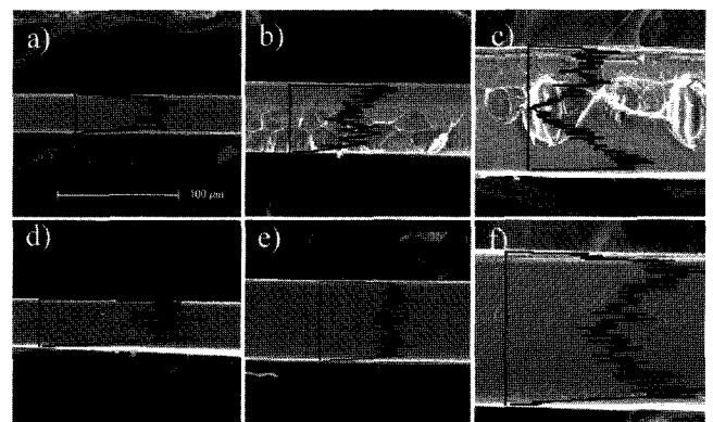
Figure 3. The relationship between the degree of grafting and the relative sulfur distribution on the cross-section of FEP-g-PSSA membranes prepared at various total irradiation doses with an irradiation dose rate of 10 kGy/h(styrene/DCM: 50/50 v/v ratio). Thicknesses of FEP films used are 25 μm(a, d); 50 μm (b, e); 100 μm (c, f), respectively.
