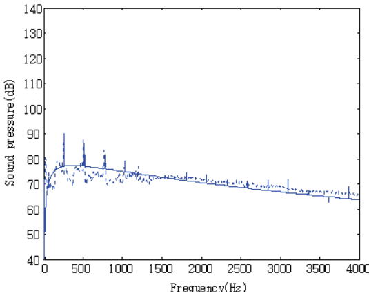
Fig. 2 Comparison of the calculated and the measured noise spectra of the bus fan(..... : measurement, ——— : prediction)
