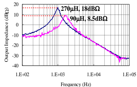
Fig. 13. Output impedance with small inductor.
