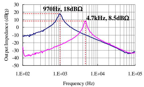
Fig. 15. Output impedance with wide bandwidth.
