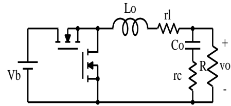
Fig. 2. POL. (buck converter)
