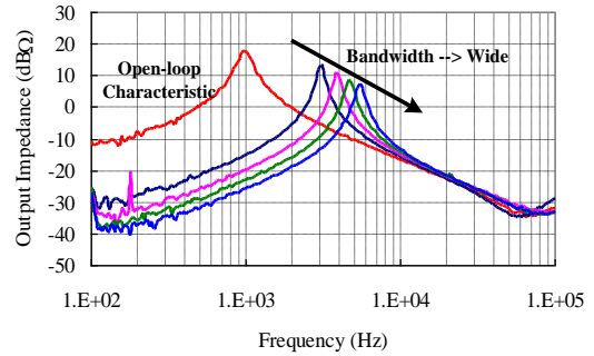
Fig. 8. Bandwidth and output impedance.
