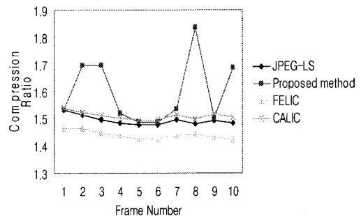
[Fig. 4] Compression ratio per frame for “Football”
