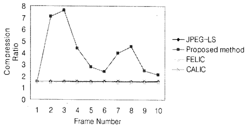
[Fig. 5] Compression ratio per frame for "Tabletennis"
