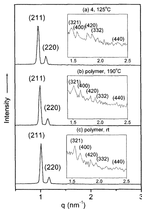
Figure 3. Small-angle X-ray diffraction patterns of (a) 4 at 125^\circ\text{C} ; (b) network polymer at 190^\circ\text{C} ; (c) network polymer at room temperature.
