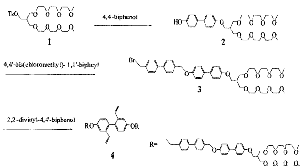
Scheme I. Synthetic route of monomer 4 .
