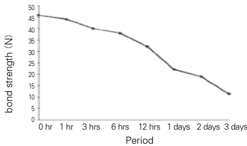
Fig. 5. Tensile bond strength (N) change according to time.
