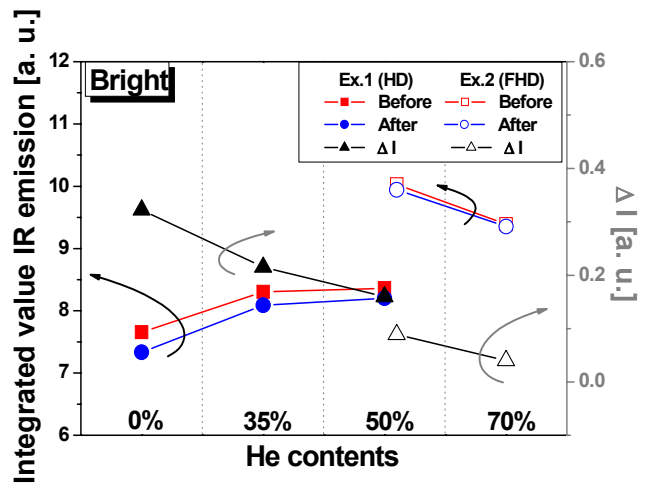
Fig. 11. Differences in the integrated IR emission of region B in Fig. 10 during the sustain period with various He contents.
