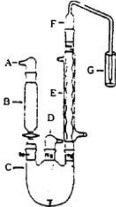
Fig. 1. Modified Monier-Williams Distillation Apparatus.
