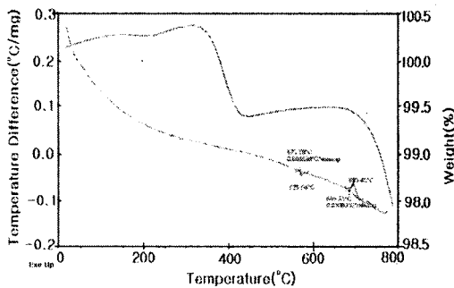
Fig. 4. TGA curve of SiO 2 /St. core-shell polymer in nitrogen(no surfactant).
