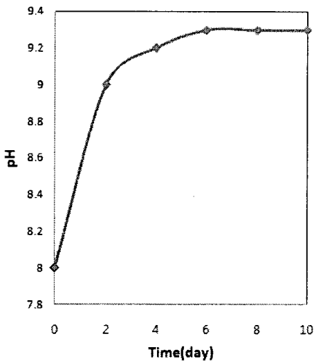
Fig. 5. Change of metal working fluid pH in the presence of copper alloy metal fiber.
