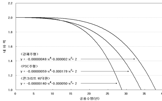
Fig. 2. Load carrying capacity curves for members.
