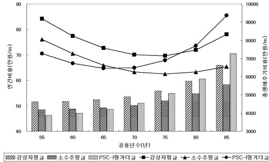
Fig. 5. Annual cost and life cycle cost of alternatives for service lives.
