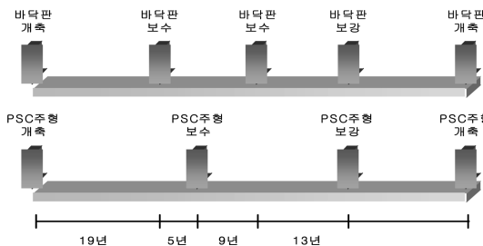
Fig. 3. Life cycle profile for PSC-I girder.
