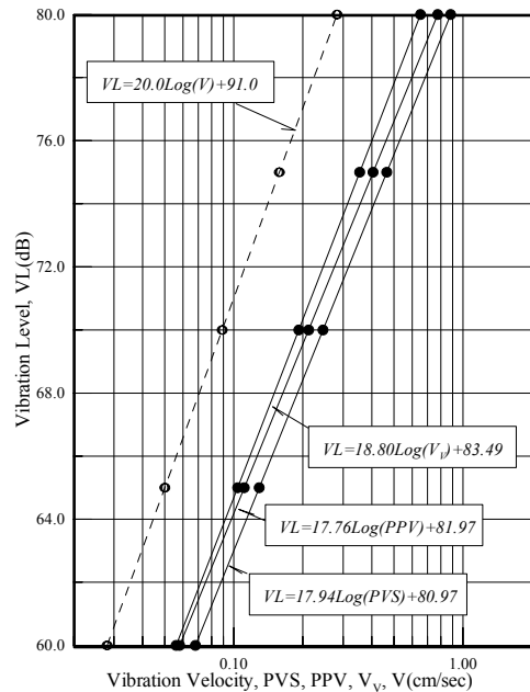
Fig. 10. Relationship between the vibration level and the vibration velocity(confidence level 97.5%).
