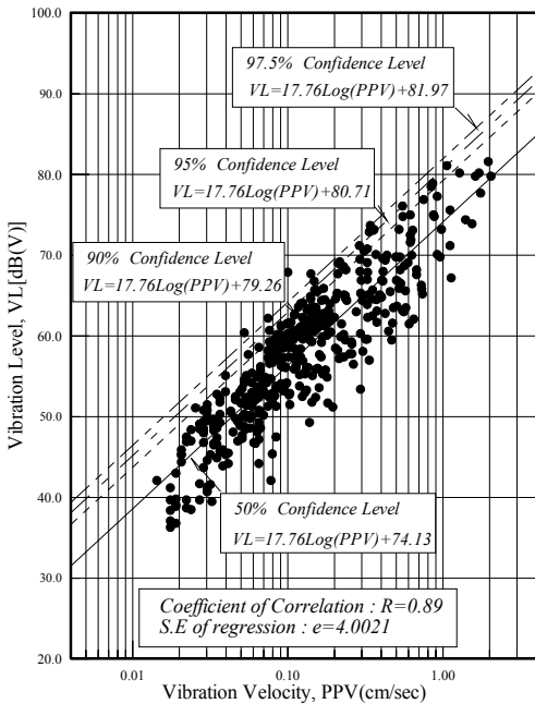
Fig. 6. Relationship between the vibration level and the vibration velocity(PPV).
