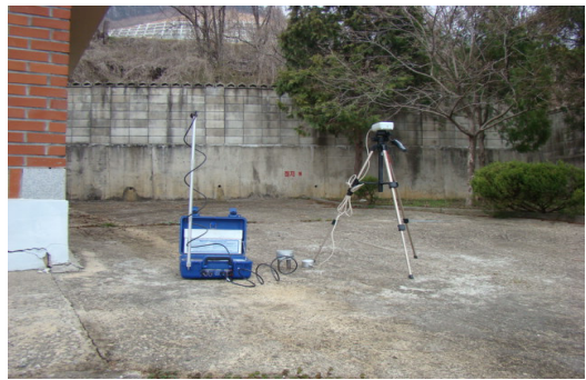
Fig. 2. Vibration monitoring on concrete.
