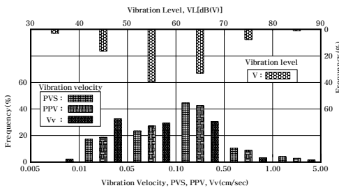
Fig. 4. Frequency distribution of the vibration level and the vibration velocity.
