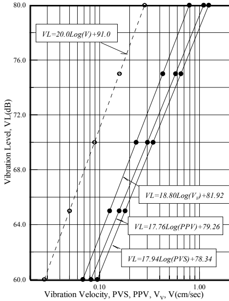
Fig. 8. Relationship between the vibration level and the vibration velocity(confidence level 90%).
