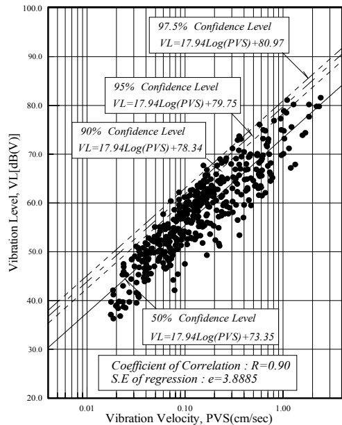
Fig. 5. Relationship between the vibration level and the vibration velocity(PVS).
