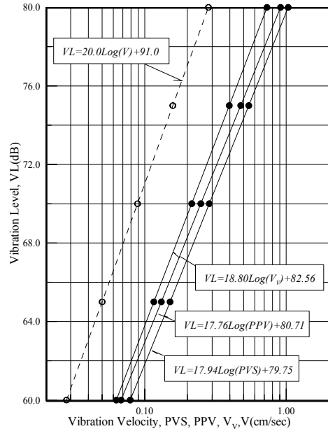
Fig. 9. Relationship between the vibration level and the vibration velocity(confidence level 95%).
