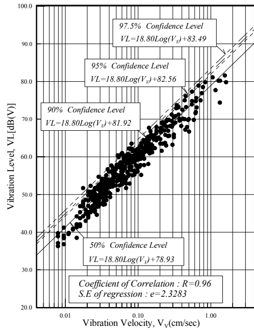
Fig. 7. Relationship between the vibration level and the vibration velocity(Vv).
