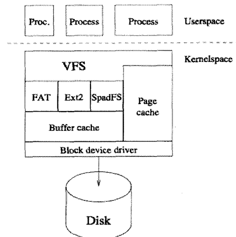
Fig. 2. File system architecture
