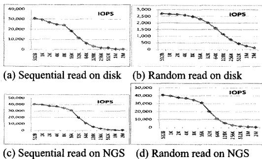
Fig. 1. Performance comparison with disk and NGS
