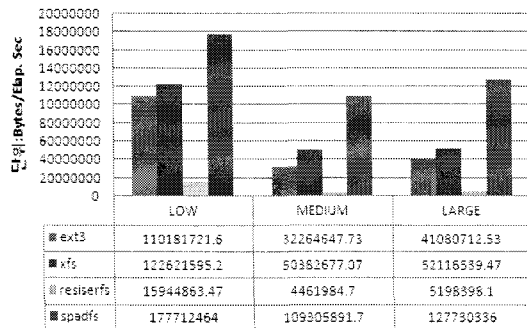
Fig. 7. Read data bandwidth
