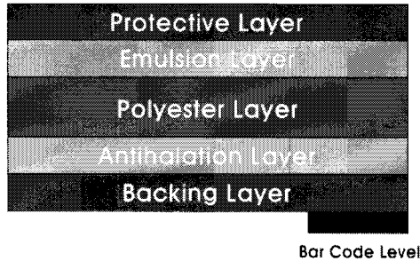
Fig. 1. IP structure
