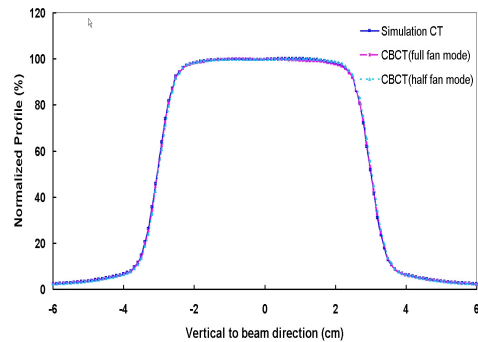
그림 7. Comparison of the dose profiles along the off-axis at the isocenter level in the homogeneous phantom
