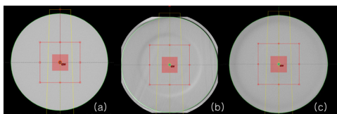
그림 5. The CT and CBCT cross section images of the Homogeneous phantom: (a) SimCT; (b) CBCTFF; (c) CBCTHF
