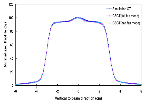
그림 8. Comparison of the dose profiles along the off-axis at the isocenter level in the Catphan-600 phantom
