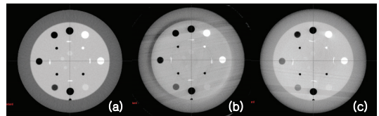
그림 4. The CT and CBCT cross section images of the Catphan-600 phantom: (a) SimCT; (b) CBCTFF; (c) CBCTHF
