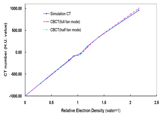
그림 6. The CT calibration curves (CT number versus relative electron density, water=1) with different image acquisition modes.
