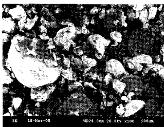
Figure 3. SEM image of unprocessed RDX particles.
