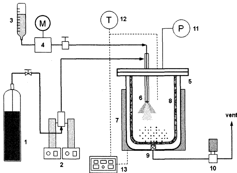
Figure 2. A schematic diagram of the experimental apparatus for SAS recrystallization.
