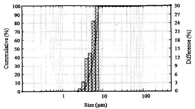
Figure 7. Particle size distribution of the RDX particles prepared at the following SAS conditions: pressure of 15 MPa, temperature of 313.15 K, RDX concentration in the feed solution of 15 wt%, CO 2 feed rate of 15 ml/min, and solution feed rate of 2 ml/min.
