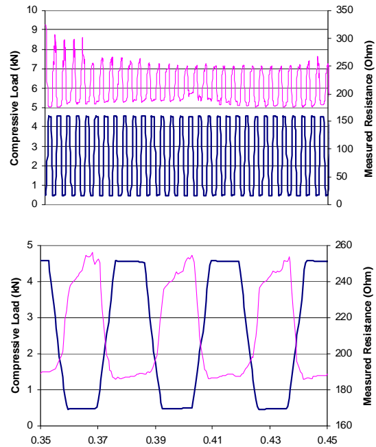
Fig. 5 Sensor (PMMA/MWNT (10 wt.% MWNT)) response to compressive cyclic loads. The sensors were constructed with conductive adhesive between copper foils and composite sensing element. Blue line represents the applied load and the pink the resulting resistance.
