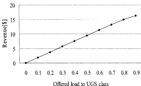
Fig. 1. Expected revenue from UGS class
