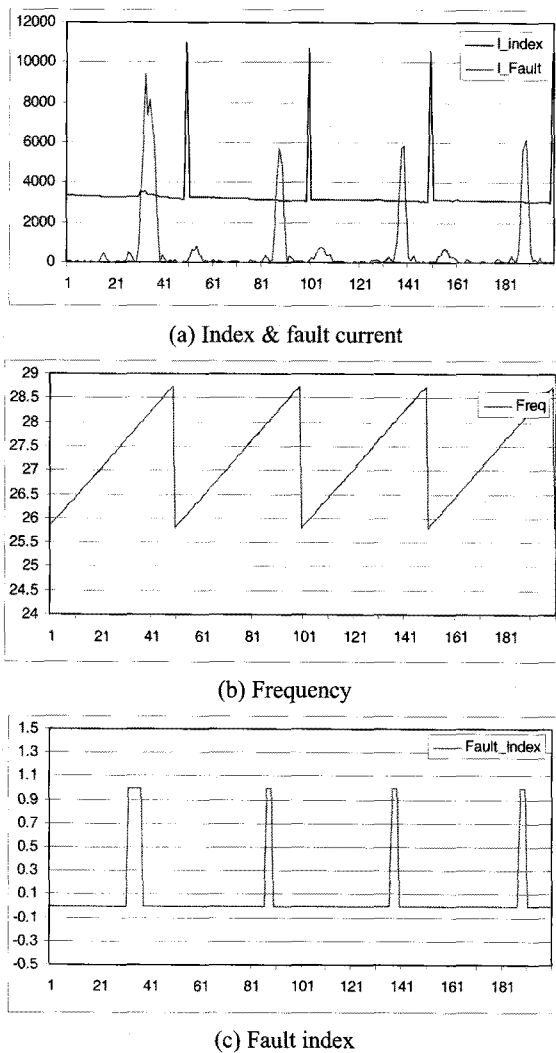
Fig. 10 Results for proposed algorithm without encoder
