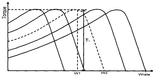
Fig. 4 Induction motor torque/speed curve
