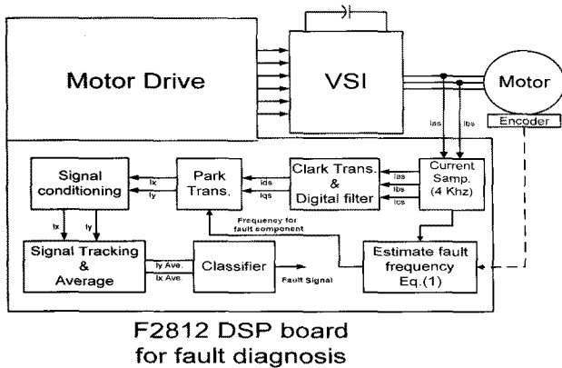
Fig. 3 System configuration
