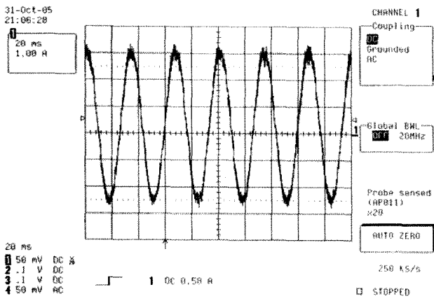
(a) Phase current waveform
