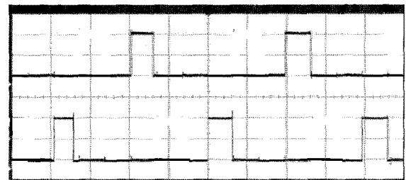
Fig. 16 Trigger signals for IGBTs S2a, S3a (upper trace: 2.5 V/div) and S1b, S4b (lower trace: 2.5 V/div) for N = 2
