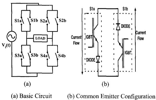
Fig. 1 Single Phase Matrix Converter
