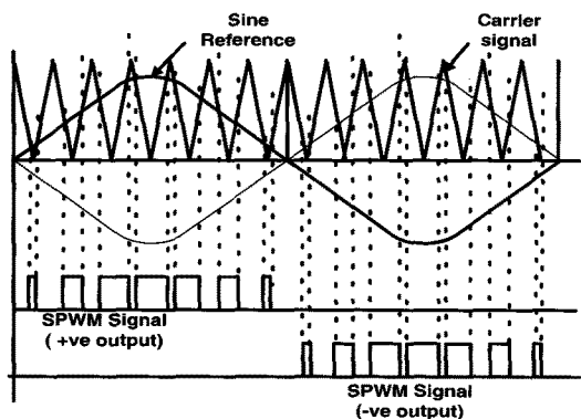
(a) SPWM
