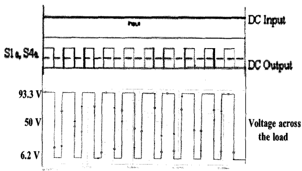
Fig. 12 Simulated Results for Chopper Operation
