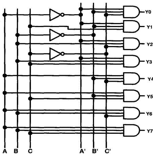
Fig. 8 Combinational Circuit
