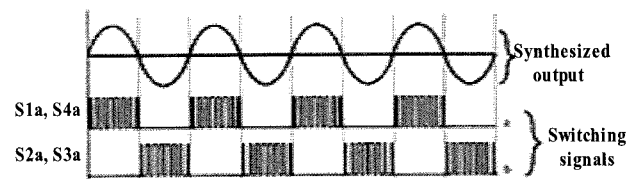
(a) Switching Pattern
