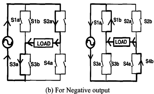
Fig 3 Cyclo Converter Operation
