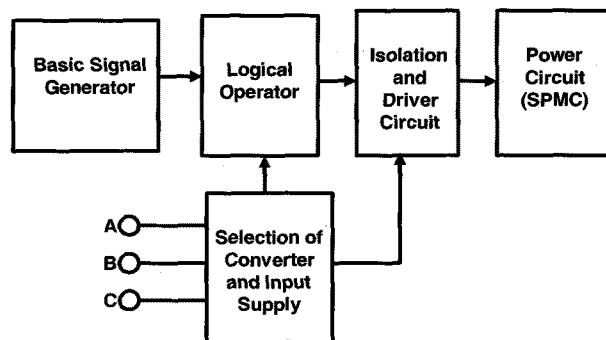
Fig. 5 Block diagram of the algorithm
