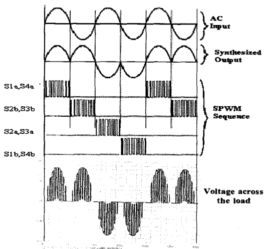
Fig. 13 Simulated Results for Cycloconverter Operation
