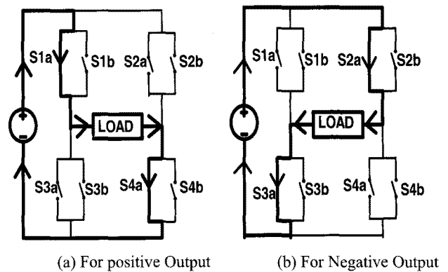
Fig. 2 Inverter operation
