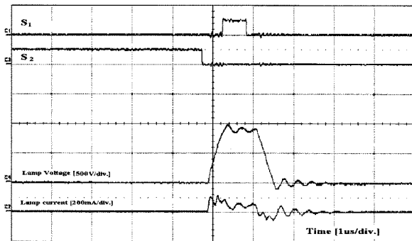
(a) Measured single pulse waveform
