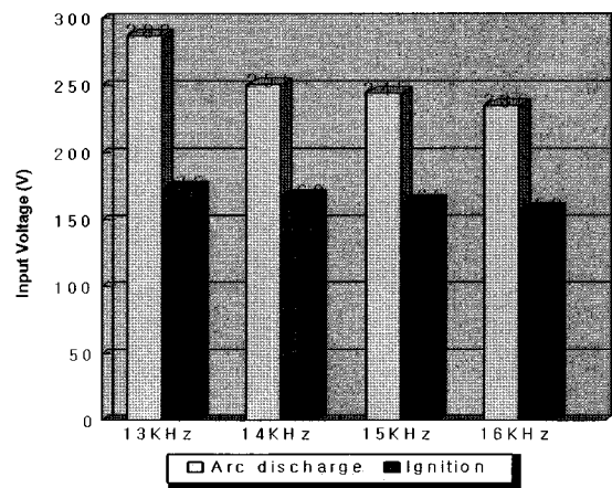
Fig. 8 Operating frequency vs. Input voltage (at 2500 \text{ cd/m}^2 )
