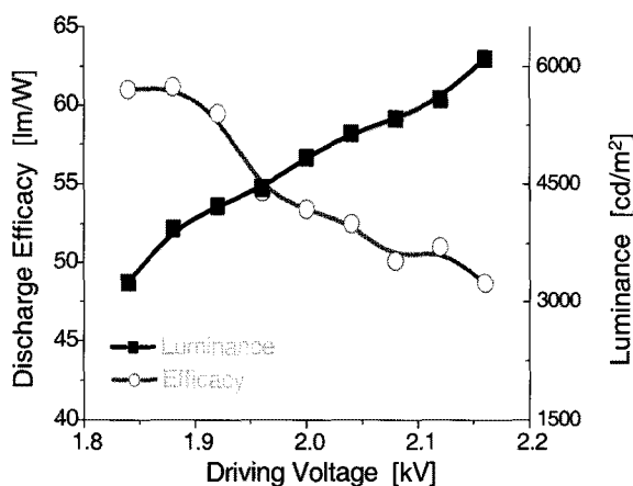
Fig. 2 The opto-electronic characteristic of high Xe content (Pulse width/interval = 1.5us/75us)
