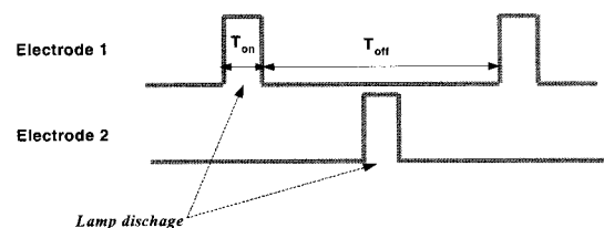
(b) Driving pulse waveforms for the lamp
