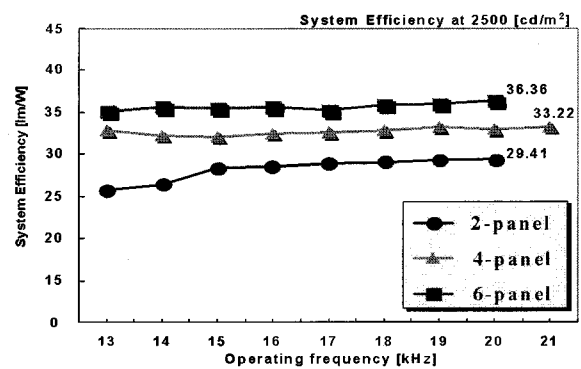
Fig. 7 System efficiency of the MFFL
