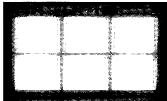
Fig. 5 A photo of 6-cell MFFL in stable glow discharge
