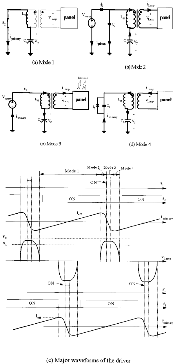
Fig. 4 Operation mode analysis and the major waveforms of the driving circuit
