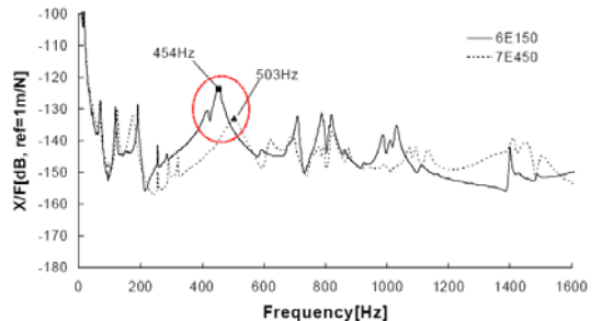
(b) Jig impact/jig response
