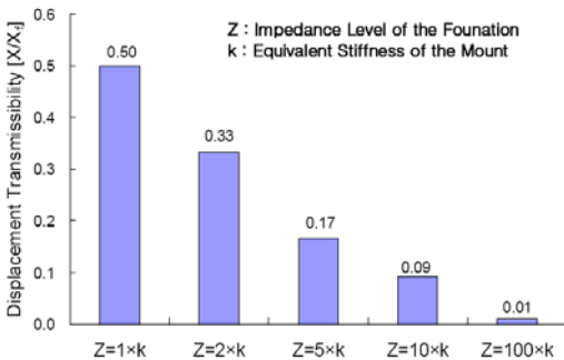
Fig. 2 Displacement transmissibility according to the impedance level of the foundation
