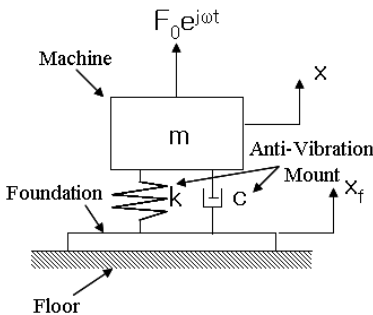
Fig. 1 2-D.O.F model for the equipment supported by resilient mount on the foundation
