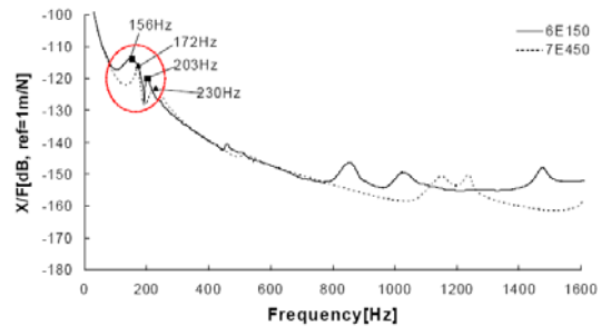
(a) Mount impact/mount response
