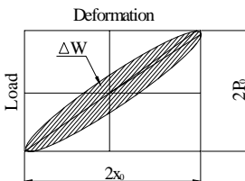
Fig. 4 Load-deformation curve for the rubber mount
