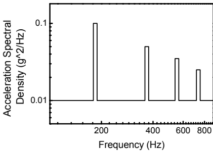
Fig. 4 Vibration exposure
