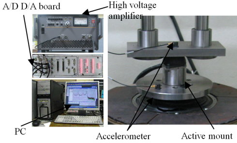
Fig. 3 Experimental apparatus for vibration control
