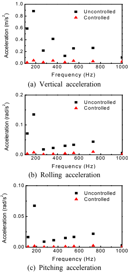
Fig. 11 Vibration control results at C.G. point
