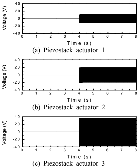
Fig. 8 Time response of the proposed camera mount system under 180 Hz excitation
