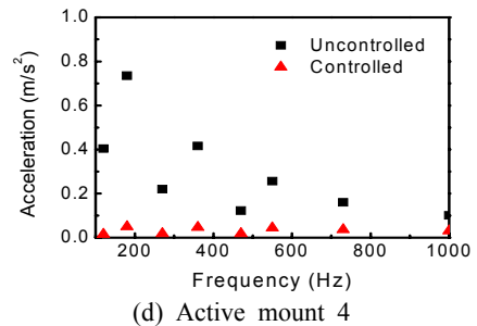
Fig. 10 Vibration control results at each mount
