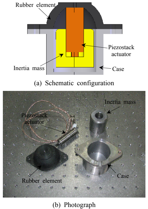
Fig. 1 Configuration of the active mount
