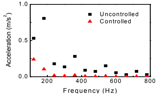
Fig. 6 Control response of the active mount in frequency domain
