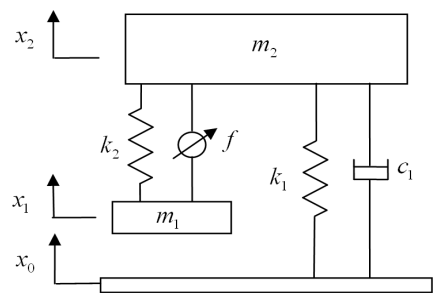
Fig. 2 Mechanical model of the active mount
