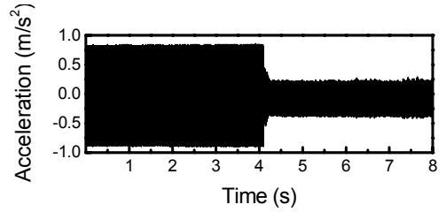
(a) Acceleration
