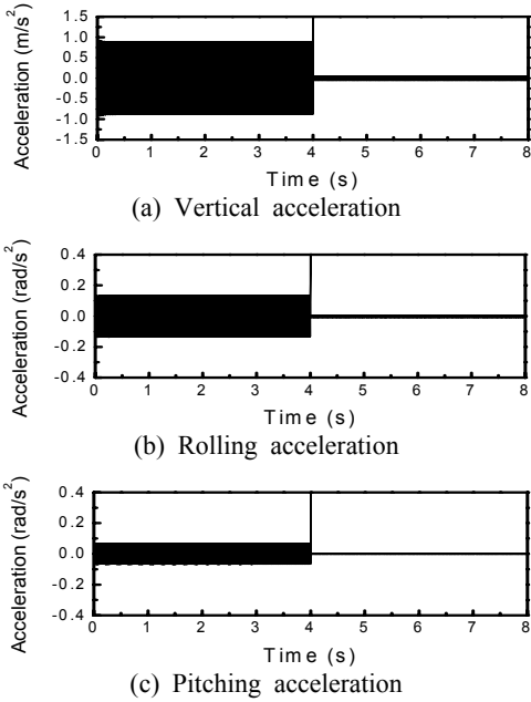
Fig. 8 Time response of the proposed camera mount system under 180 Hz excitation
