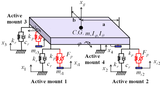
Fig. 7 Mechanical model of camera mount system
