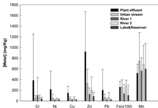
Fig. 5. Mean sediment metal concentrations (1s) by sampling site.
