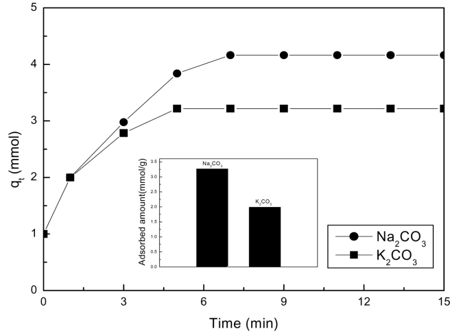
Fig. 5. Comparison of adsorption capacity between Na 2 CO 3 and K 2 CO 3 adsorbents.
