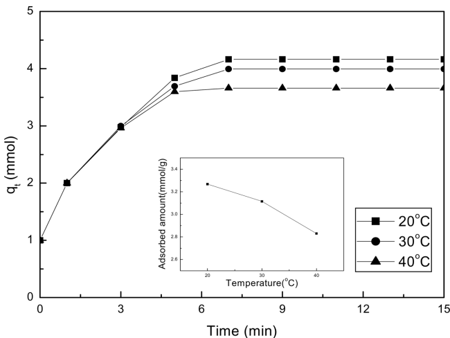
Fig. 4. Accumulations of CO 2 for different reaction temperatures.
