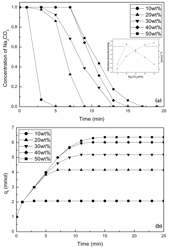
Fig. 3. Effects of Na 2 CO 3 loading on CO 2 adsorption : (a)concentration changes with reaction time, (b)accumulations of CO 2 with reaction time.
