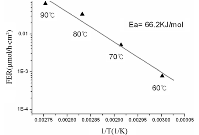
Fig. 6. Effect of cell operating temperature on the rate of chemical degradation of membrane.
