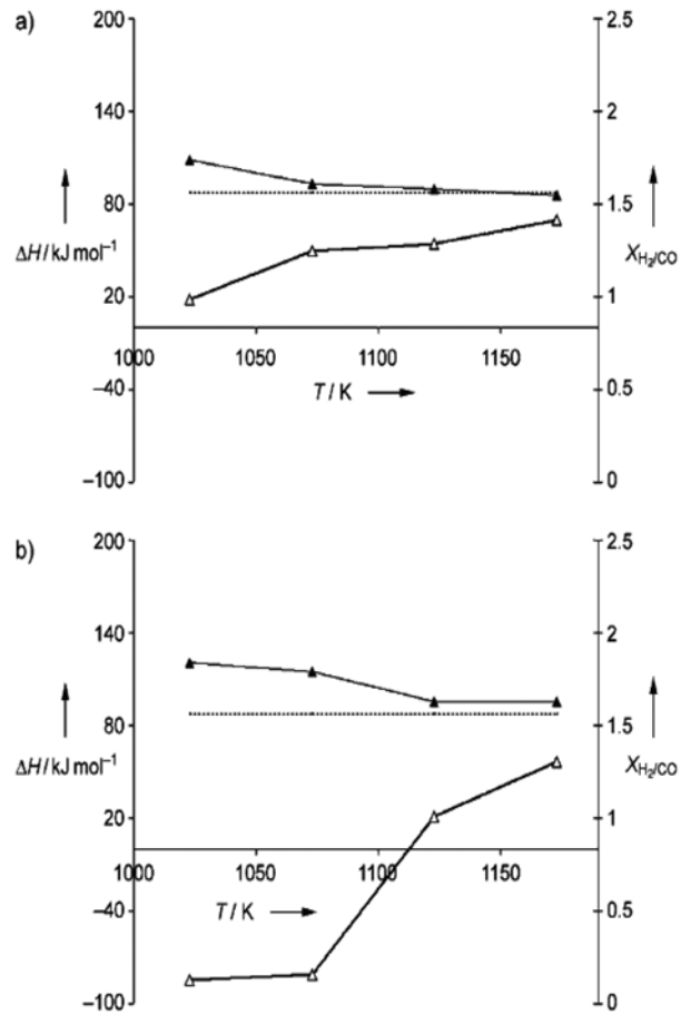
Fig. 4. Effect of temperature on the heat of reaction ( \Delta H , \Delta ) and H 2 /CO ratio [experimental ( \blacktriangle ) and equilibrium (dotted line)] during the autothermal CO 2 reforming of methane over a) CoO x /MgO/SA5205 catalyst and b) CoO x /CeO 2 /SA5205 catalyst [7].
