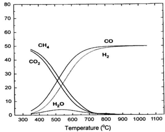
Fig. 1. Equilibrium mole fraction of CO 2 reforming as a function of temperature [11].
