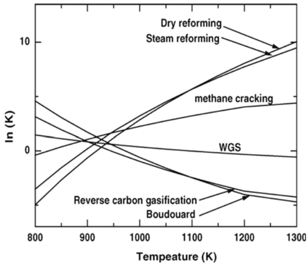
Fig. 2. Values of the equilibrium constants of reactions related to CO 2 reforming of methane [20].
