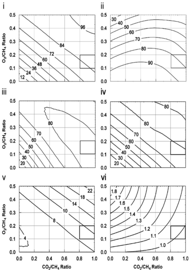
Fig. 3. Equilibrium analysis of autothermal CO 2 reforming of methane as a function of CH 4 : CO 2 : O 2 feed ratios at 1000 K for: (i) CH 4 conversions (%); (ii) CO 2 conversions (%); (iii) CO yields (%); (iv) H 2 yields (%); (v) H 2 O yields (%); and (vi) H 2 /CO ratios [49].
