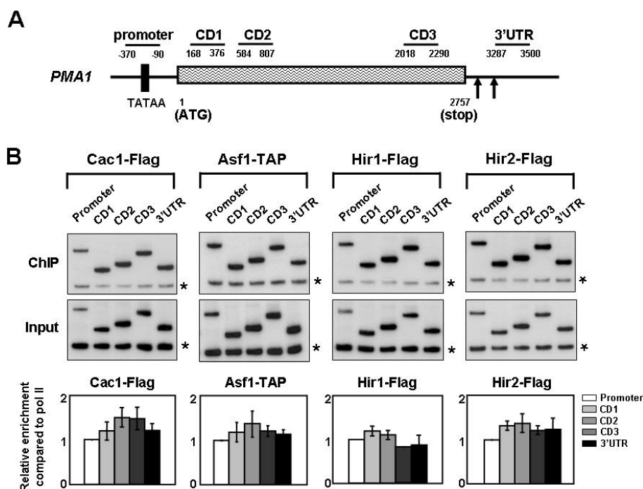
Fig. 1. The histone chaperones are associated with actively transcribed regions. (A) Schematic representation of the PMA1 locus, including primer locations for ChIP. (B) Histone chaperones are associated with the entire transcribed region of PMA1 . ChIP was performed with Asf1-TAP (YFC215), Hir1-Flag (YAG102), Hir2-Flag (YAG104), and Cac1-Flag (YAV1) using anti-Flag or IgG antibodies as described in the Materials and Methods. Representative results of at least three independent experiments are shown (Upper panel). The fold enrichment of each ChIP value was compared with that of pol II (8WG16 IP). The value obtained at the promoter region was normalized to 1 (Bottom panel). Asterisks indicate an internal control for background.
