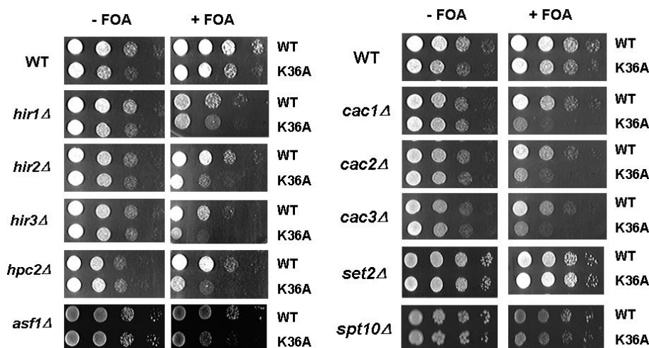
Fig. 3. The slow growth phenotype of the histone chaperone mutants in combination with the H3 K36A allele. The growth of the yeasts with deletions at the indicated gene was analyzed in combination with the H3 wild type or K36A.
