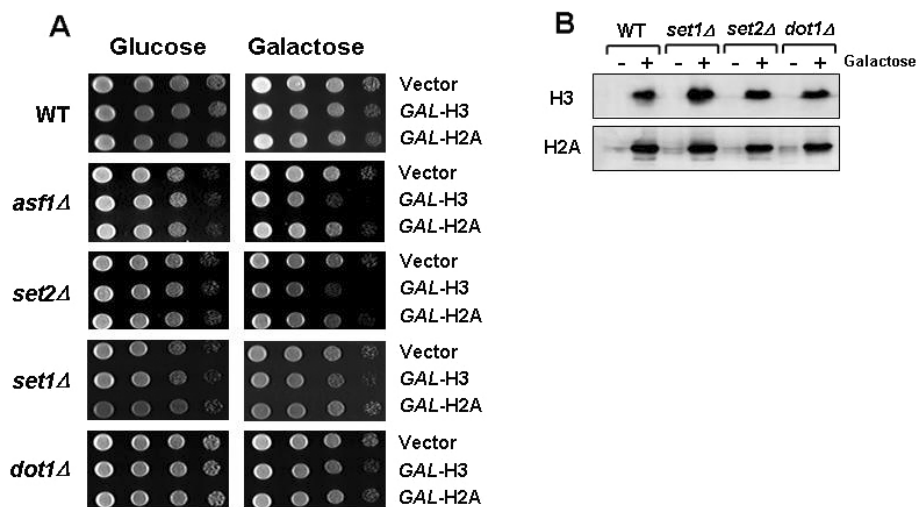
Fig. 4. The ASF1 and SET2 mutants are sensitive to over-expression of histone H3. (A) The growth of WT (BY4741), and asf1Δ , set1Δ , set2Δ , or dot1Δ mutants during overexpression of histone H2A or H3. (B) H3 or H2A were over-expressed in each strain at a similar level. The whole cell extracts prepared from the same strains in (A) were used for immunoblotting with HA-antibody.
