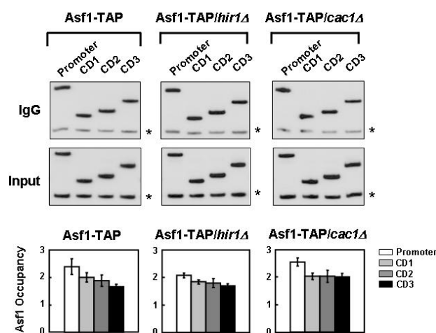
Fig. 2. Asf1 recruitment is independent of Hir1 or Cac1. ChIP was performed with yeasts expressing TAP-tagged Asf1 in the WT (YC215), hir1Δ (YC204), or cac1Δ (YC205) as described in Fig. 1 (Upper panel). Each PCR signal was normalized to the intergenic control and the input signal (Bottom panel).
