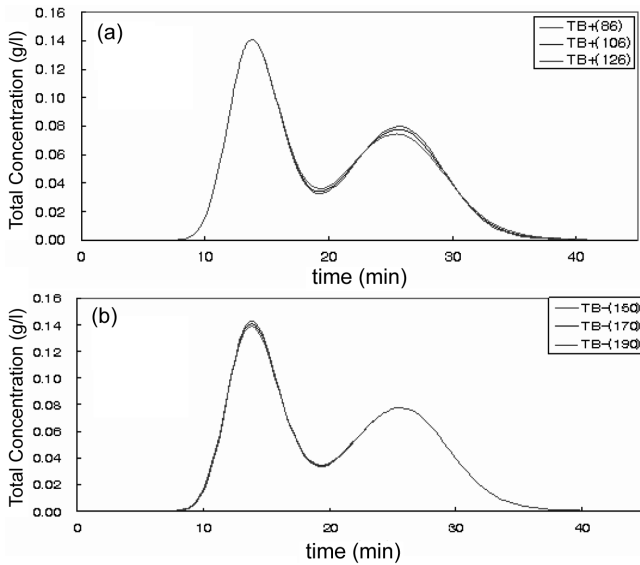
Fig. 9. Variation of chromatograms according to the increase of number of plates (a) TB(+), (b) TB(-).
