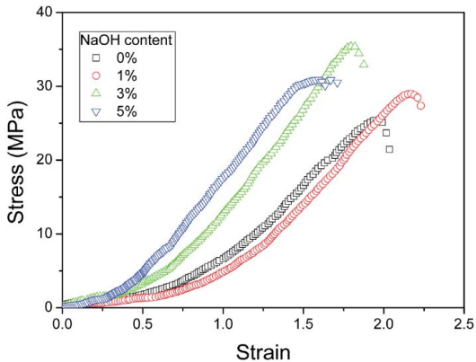
Fig. 8. Tensile stress-strain diagram of PP/kenaf bio-composite (70/30 wt%).
