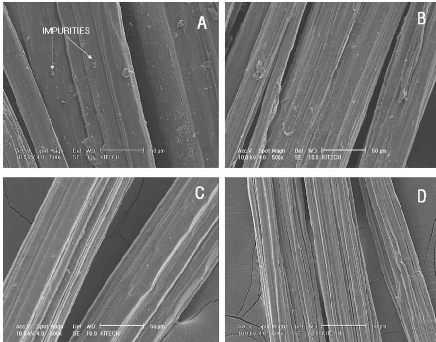
Fig. 6. SEM micrographs of the (A) an untreated kenaf fiber and (B) 1% NaOH treated (C) 3% NaOH treated (D) 5% NaOH treated : 50 \mu\text{m} ( \times 500 ).
