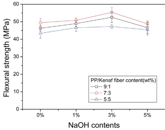
Fig. 9. Flexural strength of PP/kenaf bio-composite.
