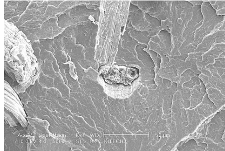
Fig. 13. SEM micrographs of PP/3% NaOH treated kenaf fiber (70/30) interface on bio-composite: 50 \mu\text{m} ( \times 500 ).
