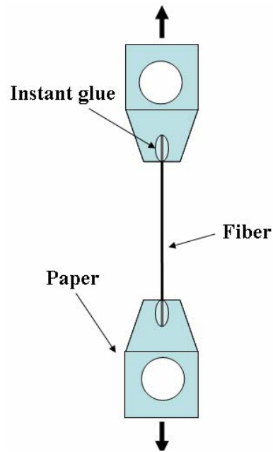
Fig. 2. The schematics of fiber tensile test.
