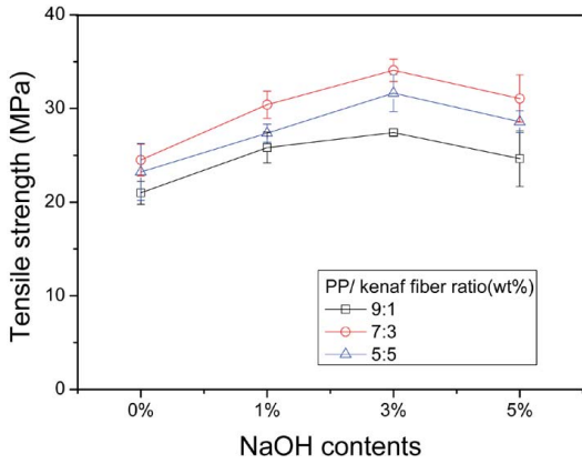
Fig. 7. Tensile strength of PP/kenaf bio-composite.
