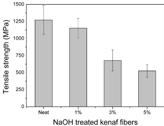
Fig. 4. Tensile strength of NaOH treated kenaf fibers.
