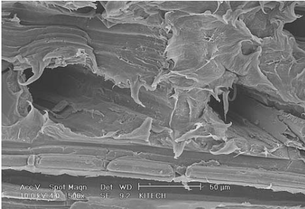
Fig. 11. SEM micrographs of PP/untreated kenaf fiber (70/30) interface on bio-composite: 50 \mu\text{m} ( \times 500 ).
