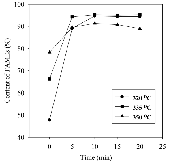
Fig. 3. Effect of reaction time and temperature on the content of FAMES at 20 MPa, 45:1(molar ratio).
