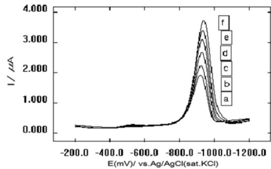
Fig. 4. SW voltammograms of ranitidine · HCl in the sample solution and standard added solutions.
