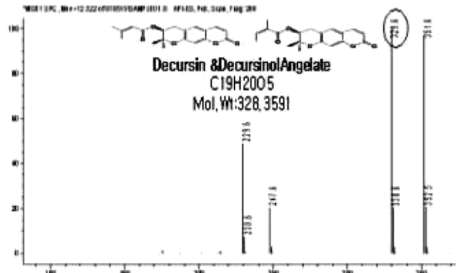
Fig. 1. LCMS plot of root extracts of Angelica gigas Nakai.
