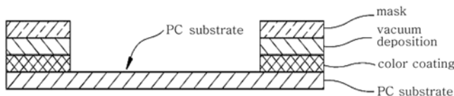
Fig. 4. Schematic diagram of cross-section of window lens.
